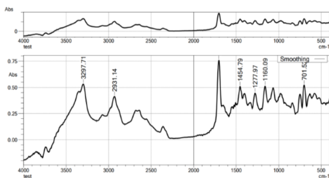
Figure 3: FT-IR spectra of Physical Mixture
