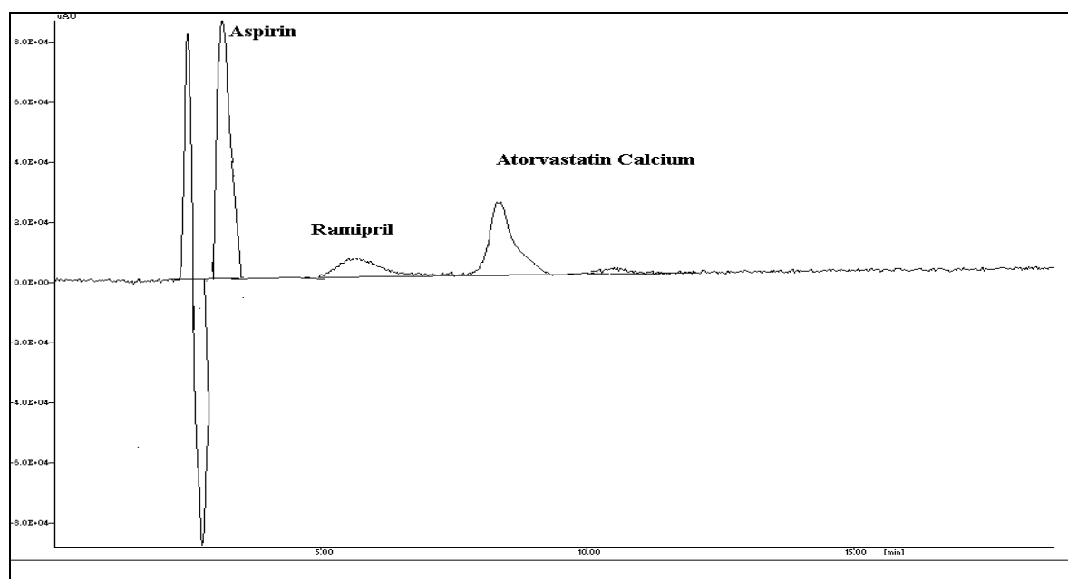
Figure 1: A Representative Chromatogram of Aspirin, Ramipril and Atorvastatin Calcium at 210 nm
