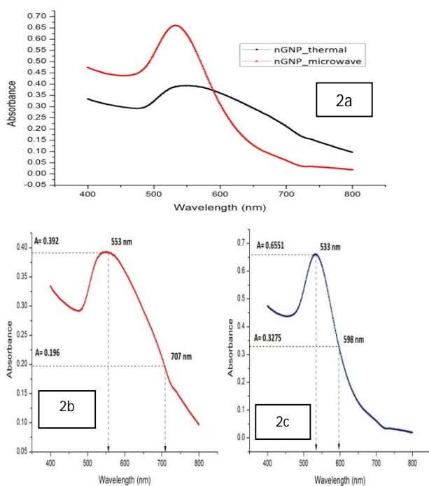
Figure 2: (a) Absorption spectrum of A.indica GNPs synthesized by two different heating techniques; i.e. microwave and conventional hot plate heating, (b) and (c) Area under the curve of GNPs synthesized by
